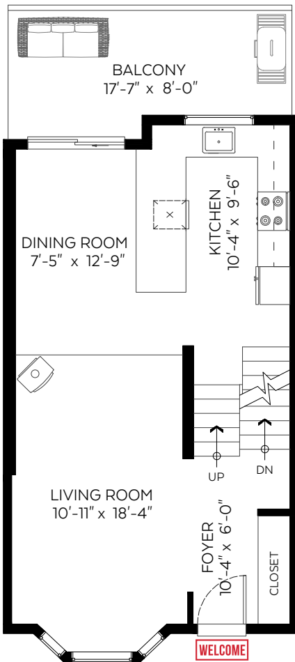
Main Floor Plan Floor Area: 582 sq.ft. Ceiling Height: 8 ft.
