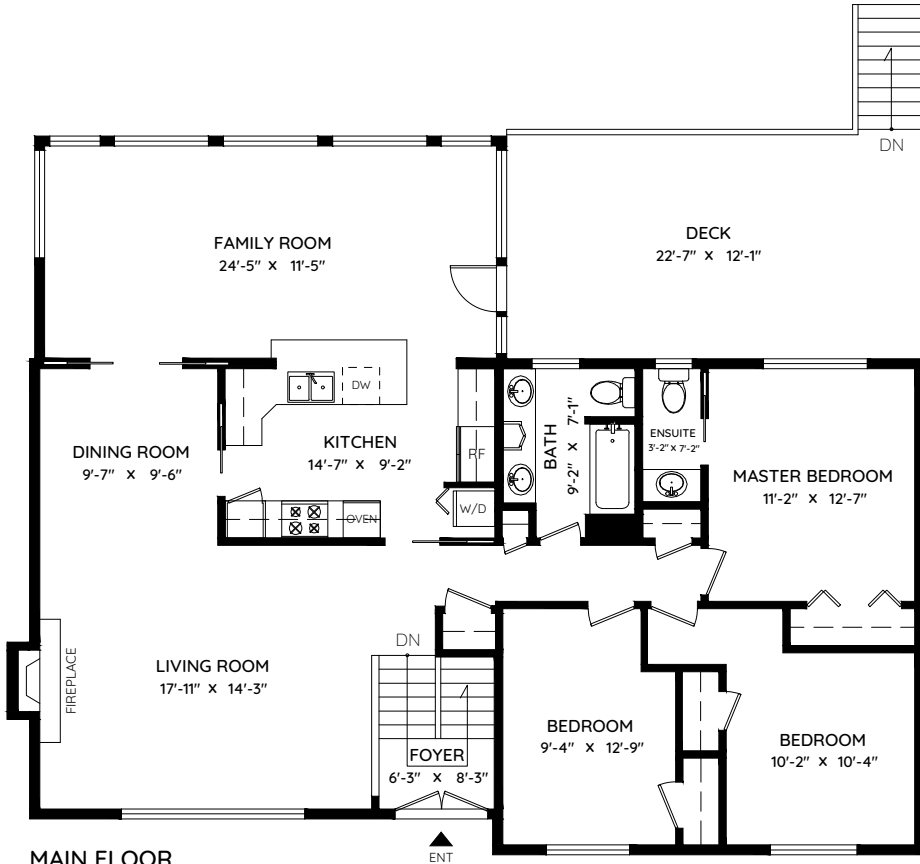
MAIN FLOOR 1,551 SQ.FT. CH: 8'-0"
