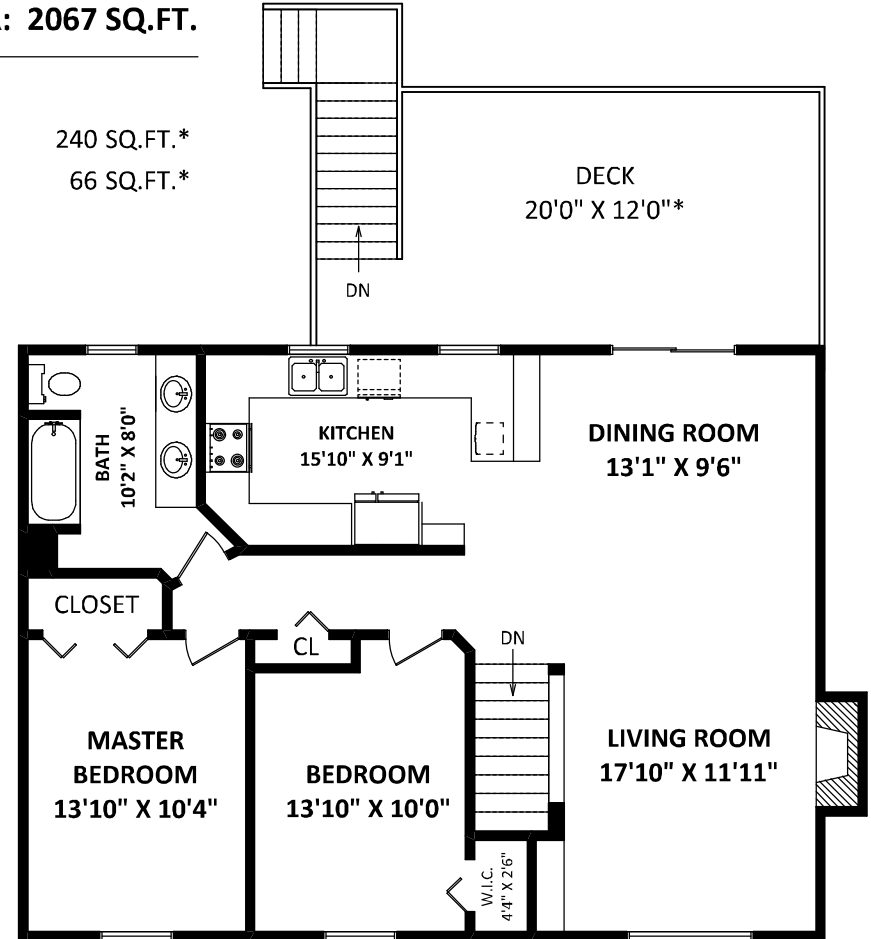
MAIN FLOOR: 1075 SQ.FT.
