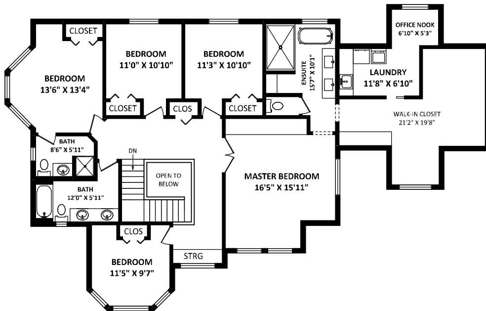
UPPER FLOOR: 1992 SQ.FT.
