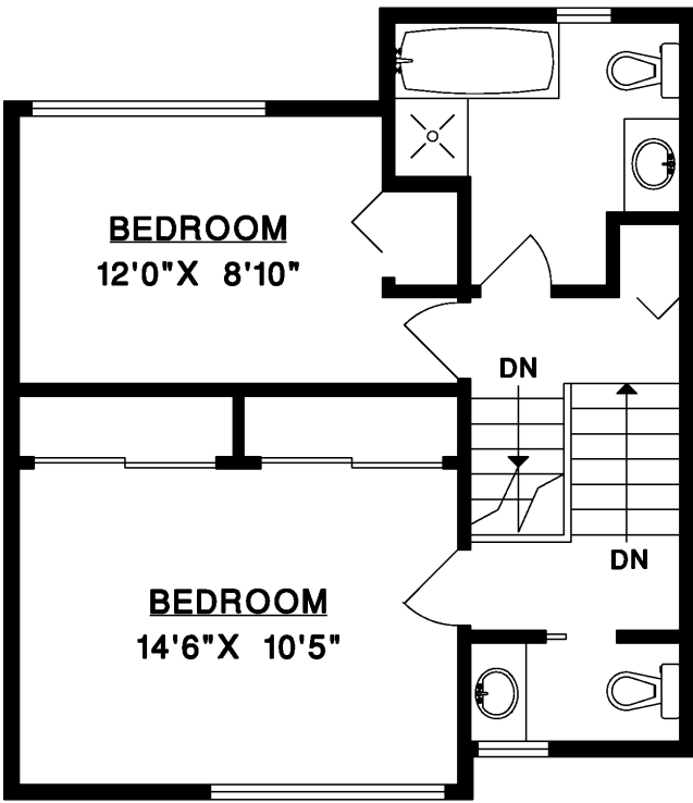
UPPER FLOOR
