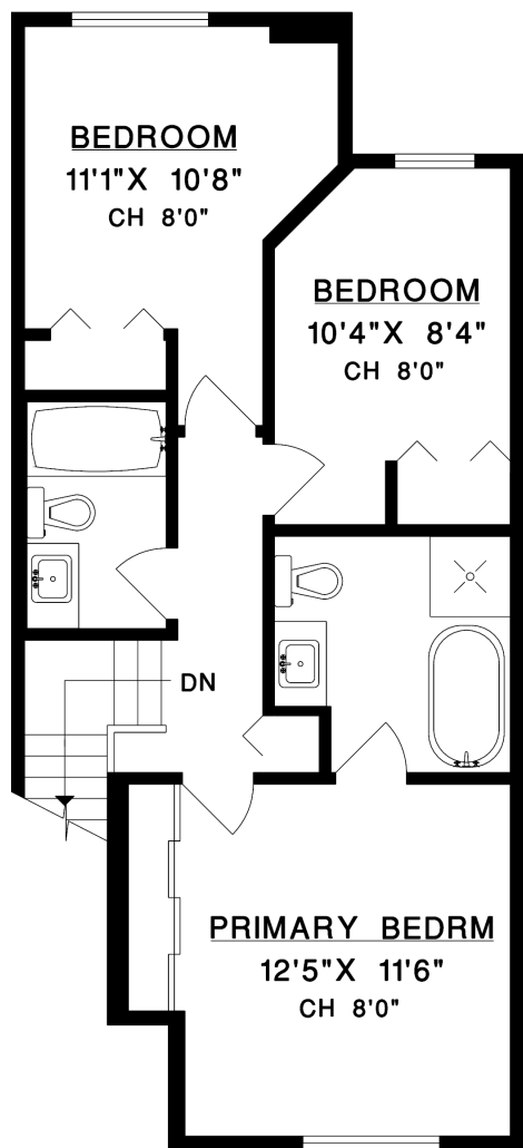
UPPER FLOOR
