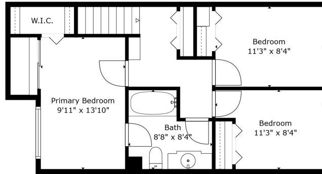
Upper Floor - Ceiling Height: 8'
