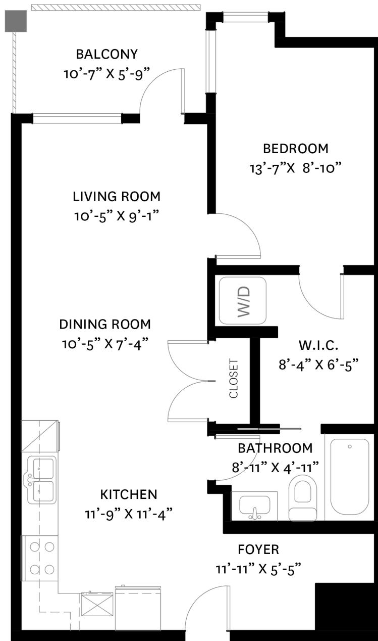
MAIN FLOOR PLAN Ceiling Height: 9'-0"
