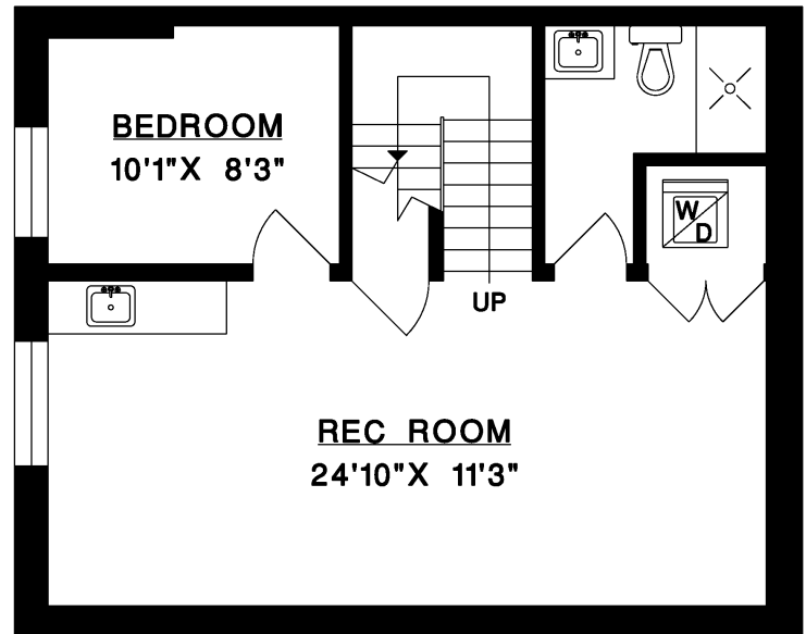
LOWER FLOOR
