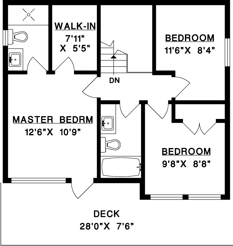
UPPER FLOOR
