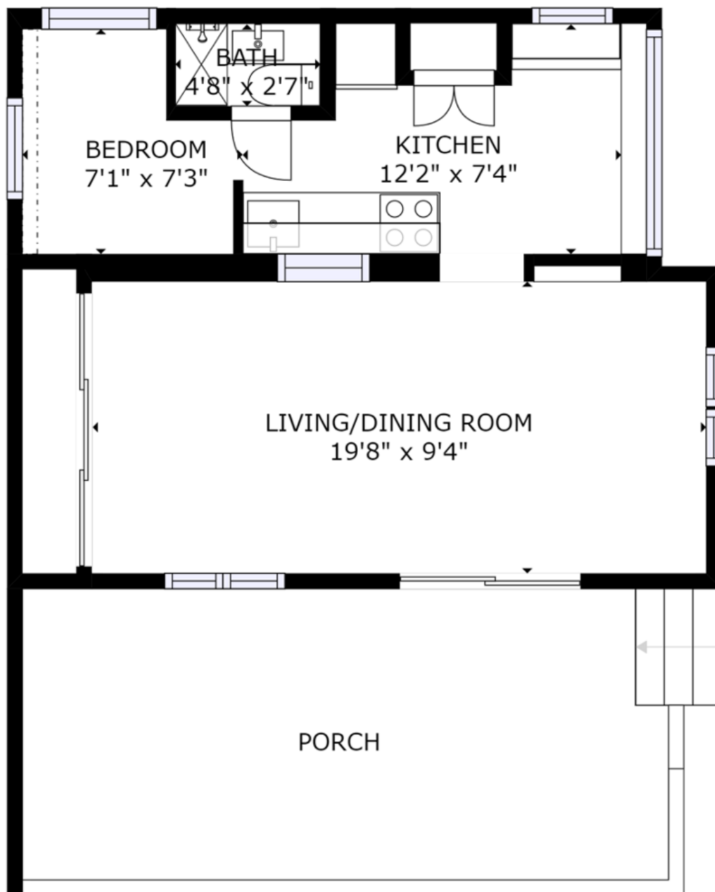
FLOOR 1
