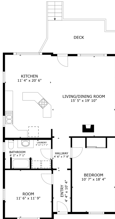
FLOOR PLAN
