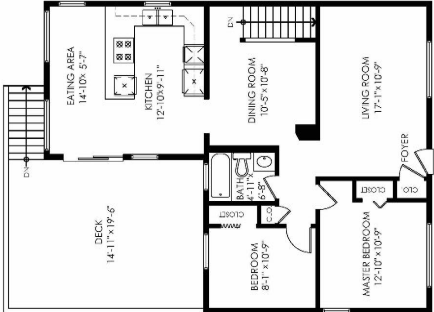
Main Floor Plan Floor Area: 968 sq.ft. Ceiling Height: 8'
