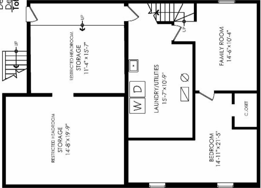
Lower Floor Plan Floor Area: 771 sq.ft. Ceiling Height: 7'
