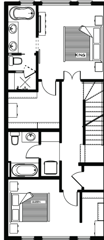
3RD FLOOR
