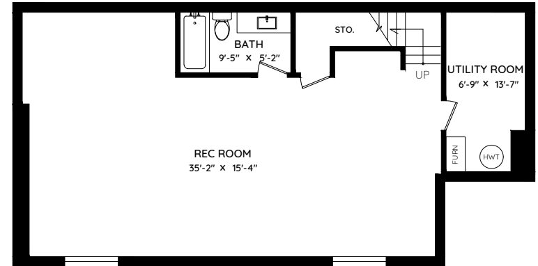
LOWER FLOOR 950 SQ.FT. CH: 8'-2"
