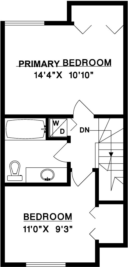
UPPER FLOOR
