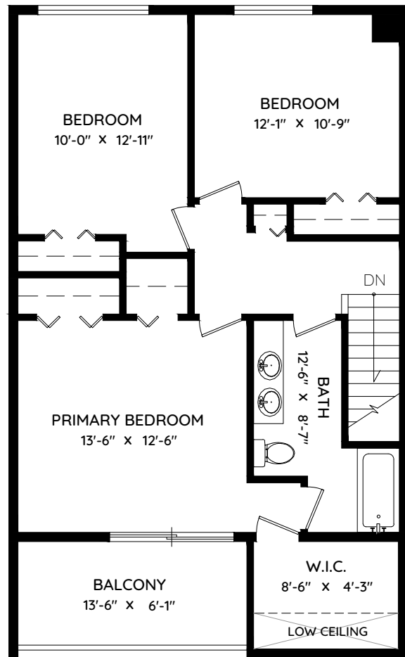
UPPER FLOOR 784 SQ.FT. CH: 8'-0"
