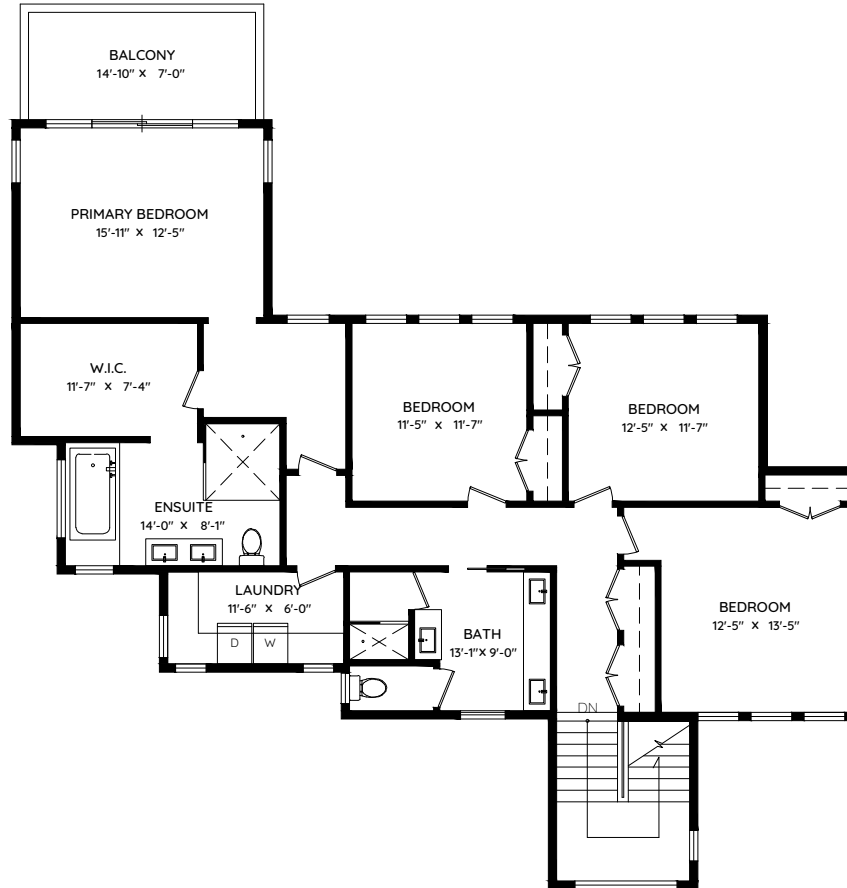
UPPER FLOOR 1,599 SQ.FT. CH: 8'-0"
